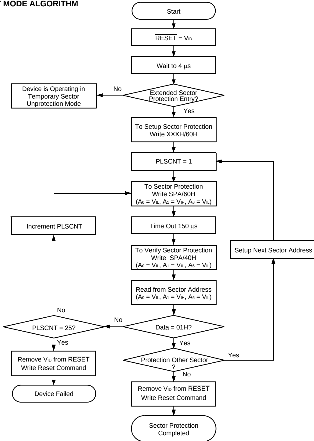
Figure 23 Extended Sector Protection Algorithm
