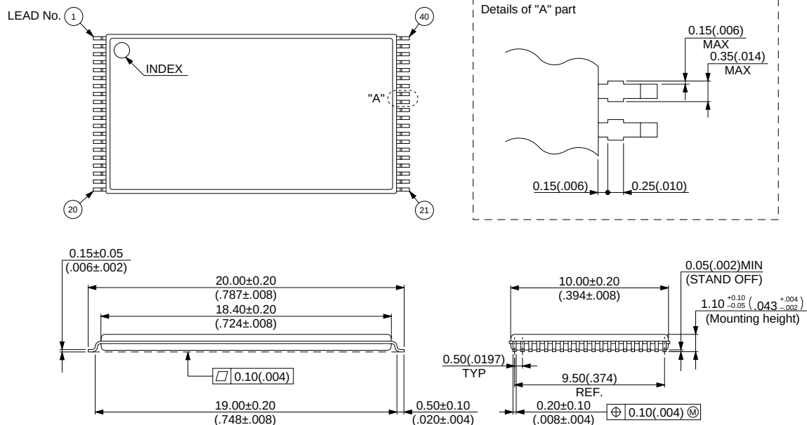
40-pin plastic TSOP(I) (FPT-40P-M06)
